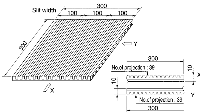
Square Type (PT-1030)
