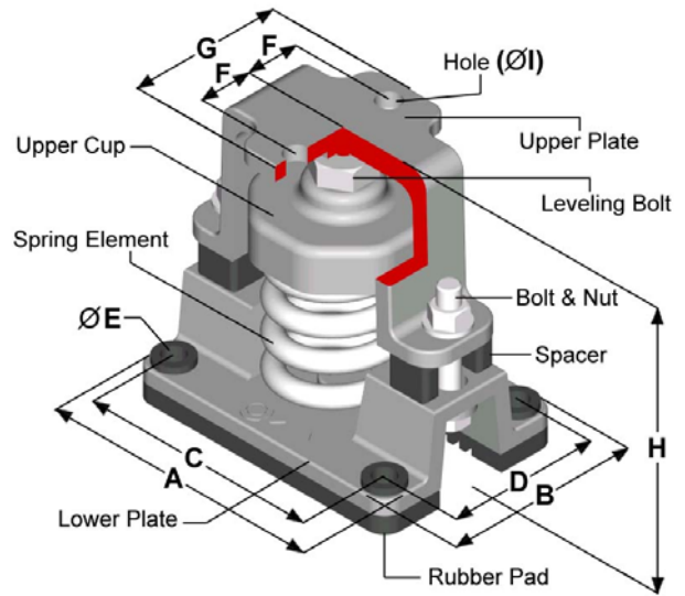
PTM-D-451M, 601EM, 826EM, 1101EM, 1401EM PTM-D2-176, 246, 351, 526, 751, 1051
