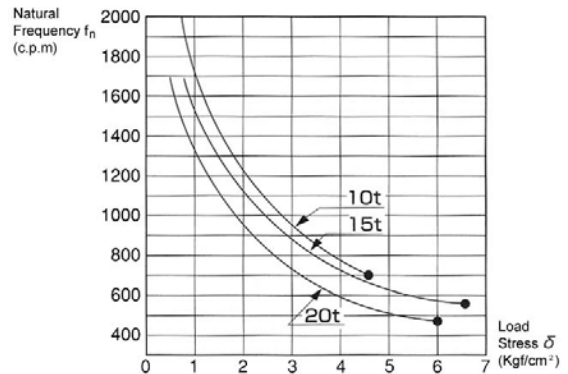
Fig.2 Characteristic of Natural Frequency-Load Stress
