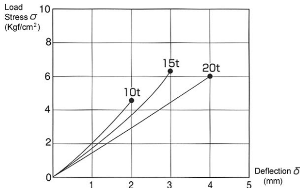
Fig.1 Characteristic of Load Stress-Deflection
